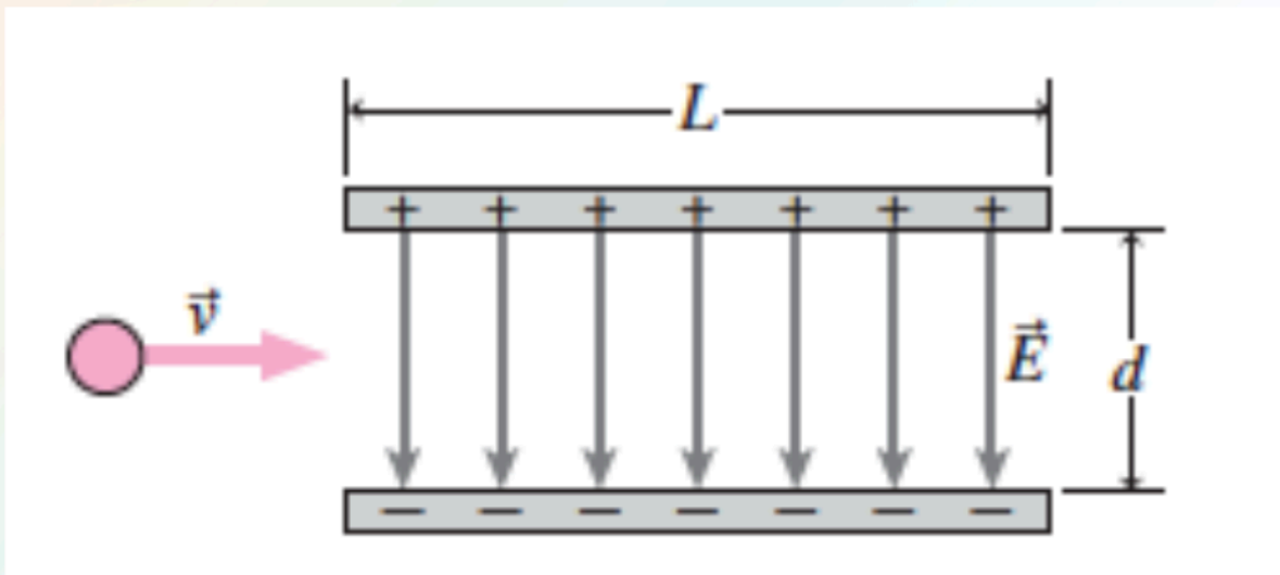
Figure 10. Electron moves in a Uniform Electric Field. From. Essential University Physics (pp 350) by Wolfson R.(2012). Addison-Wesley, Pearson
