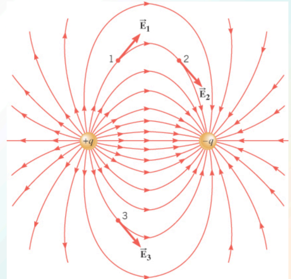
Figure 8. Electric Field Lines leaving a positive charge or entering a negative charge.. Retrieved from https://courses.lumenlearning.com/physics/chapter/18-5-electric-field-lines-multiple-charges/
