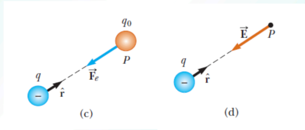
Figure 12. c) Force on a Test Charge. d) Electric Field of a Test Charge From. Physics for Scientists and Engineers with Modern Physics (pp 700) by Serway, R. A., & Jewett, J. W. (2019). Australia: Cengage Learning.
