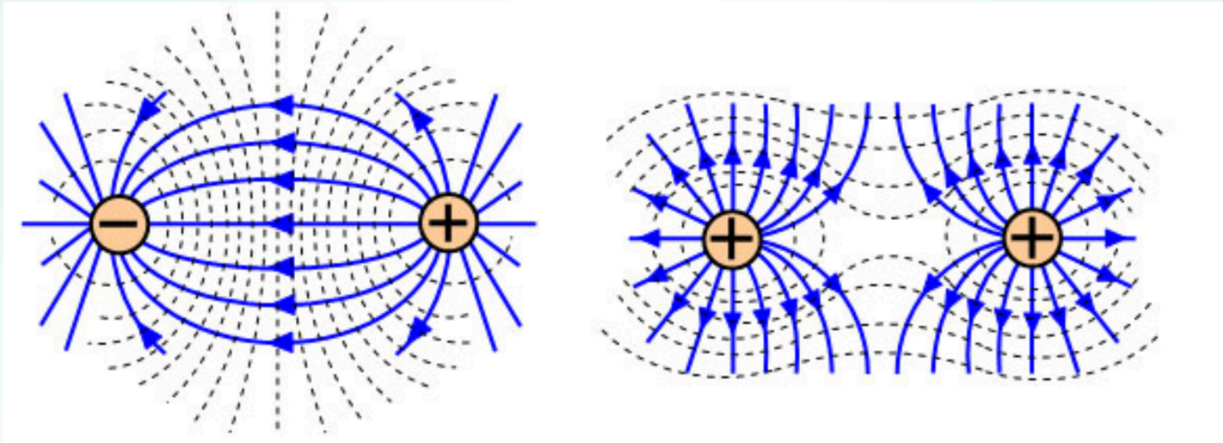
Figure 2. Electric Field Lines. Retrieved from https://brilliant.org/wiki/electric-field-lines/
