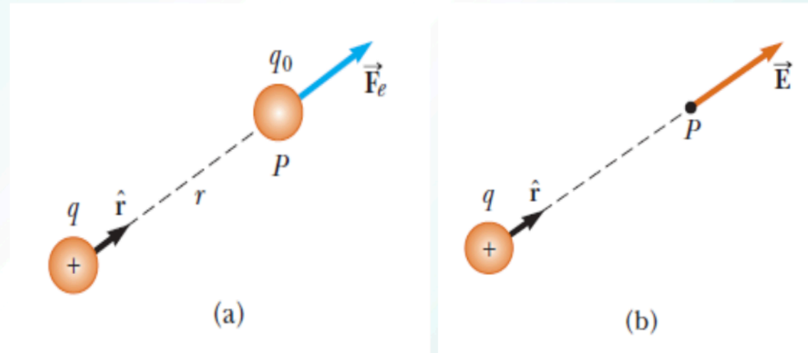
Figure 12. a) Force on a Test Charge. b) Electric Field of a Test Charge From. Physics for Scientists and Engineers with Modern Physics (pp 700) by Serway, R. A., & Jewett, J. W. (2019). Australia: Cengage Learning.
