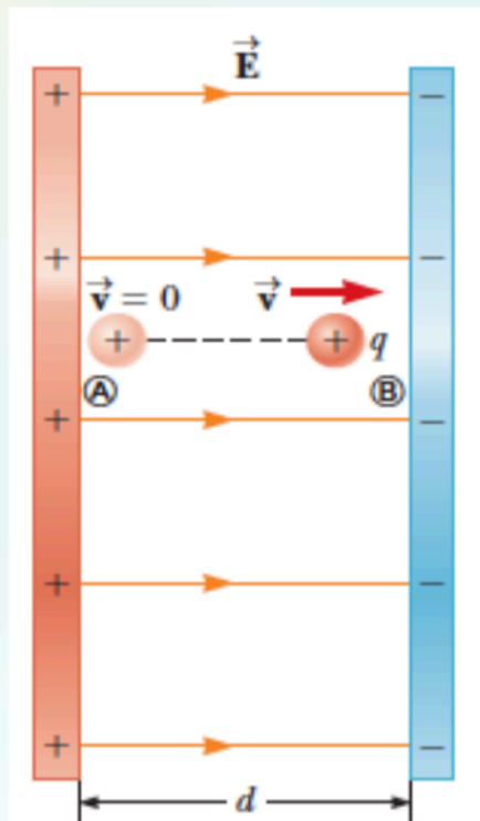
Figure 11. A positive point charge in a uniform electric field. From. Physics for Scientists and Engineers with Modern Physics (pp 711) by Serway, R. A., & Jewett, J. W. (2019). Australia: Cengage Learning.
