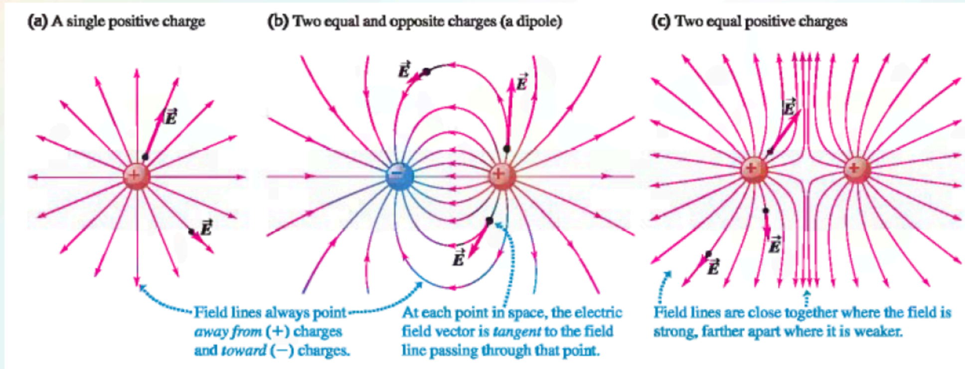
Figure 5. Electric field lines for three different charge distributions. From Sear's & Zemansky's University Physics With Modern Physics (pp 699) by Young, H. D., Freedman, R. A. & A. Lewis Ford (2016). England: Pearson.
