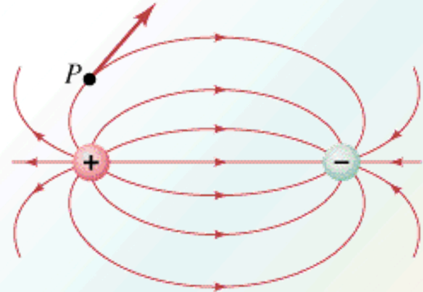
Figure 6. Electric Field Lines due to two equal charges of opposite signs. Retrieved from https://courses.lumenlearning.com/physics/chapter/18-5-electric-field-lines-multiple-charges/
