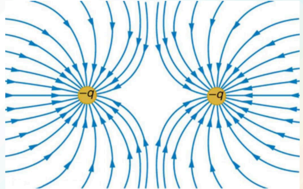
Electric field lines for 2 EQUAL NEGATIVE charges
