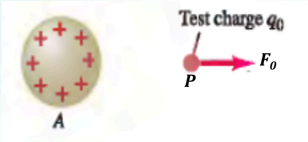
Figure 1. c) A charged body creates an electric field in the space around it. From: Sear's & Zemansky's University Physics With Modern Physics (pp 699) by Young, H. D., Freedman, R. A. & A. Lewis Ford(2016). England: Pearson
