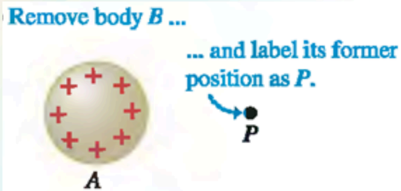
Figure 1. b) A charged body creates an electric field in the space around it. . From: Sear's & Zemansky's University Physics With Modern Physics (pp 699) by Young, H. D., Freedman, R. A. & A. Lewis Ford(2016). England: Pearson.
