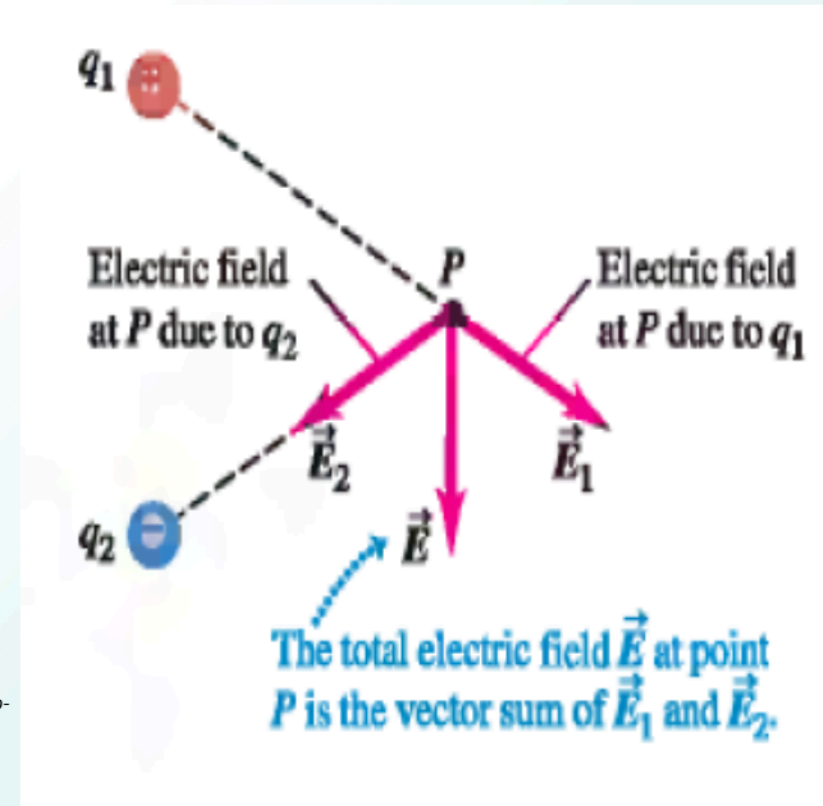
Figure 13. The total electric field. From. https://www.miniphysics.com/wp-content/uploads/2010/11/electric-field-between-point-charges.png
