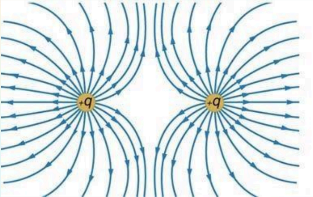
Electric field lines for 2 EQUAL POSITIVE charges
