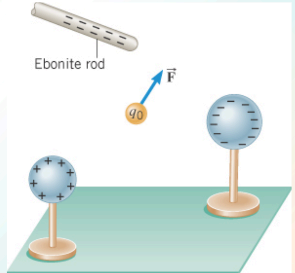
Figure 3. Electric Field. Retrieved from http://physicsskills.pbworks.com/f/E%2BForces%2Band%2BE%2BFields.pdf
